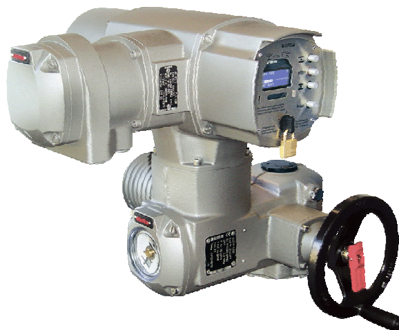
AUMA SA multi-turn actuator with AUMATIC actuator controls
